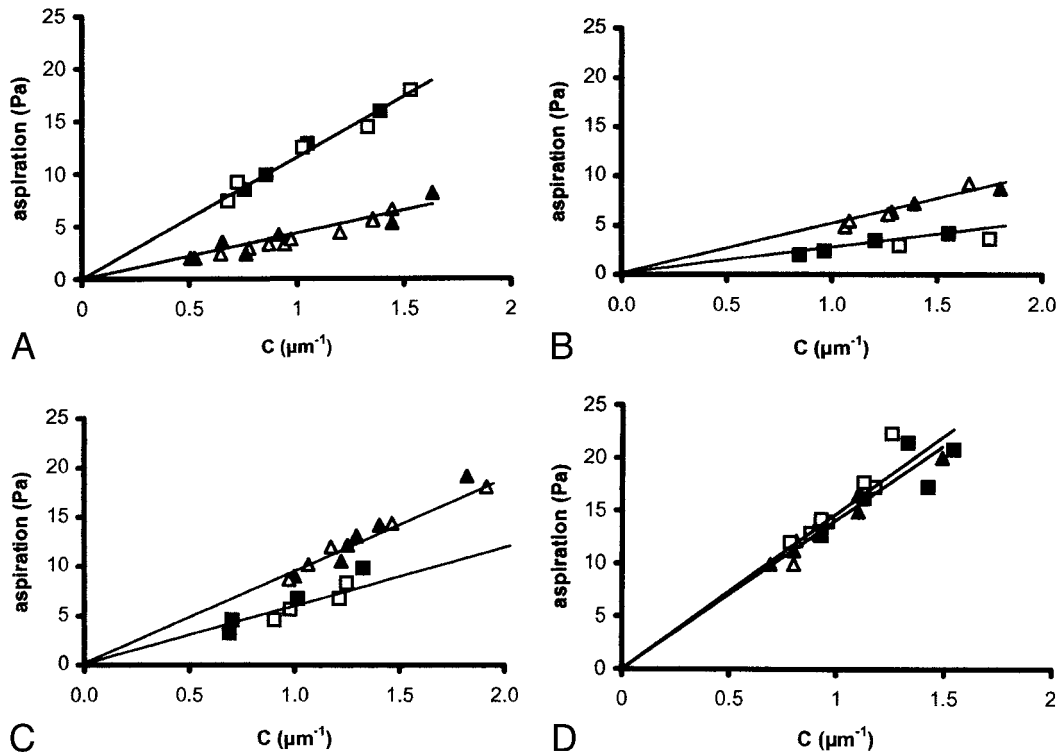
FIGURE 3 Aspiration pressure as a function of parameter C given in Eqs. 3 and 4. (a) \text{Le}^x/\text{Le}^x experiment (two vesicles with \text{SOPC}:\text{Le}^x of 90:10); (b) \text{Lex}/\text{Lac} experiment (one vesicle is \text{SOPC}:\text{Le}^x 90:10; the other is \text{SOPC}:\text{Lac} 90:10); (c) \text{Lac}/\text{Lac} experiment (two vesicles with \text{SOPC}:\text{Lac} 90:10); (d) pure SOPC vesicles. The closed symbols represent decreasing aspiration, and open ones represent increasing aspiration. Triangles are for \text{NaCl} solution and squares for \text{CaCl}_2 . The straight lines are least-squares fits.
